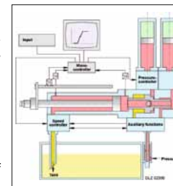
Opticast casting unit
